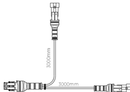
ZONE 6 - Superseal Y-kabel 1x female 2x male 300cm (Art. KS1-6300)
